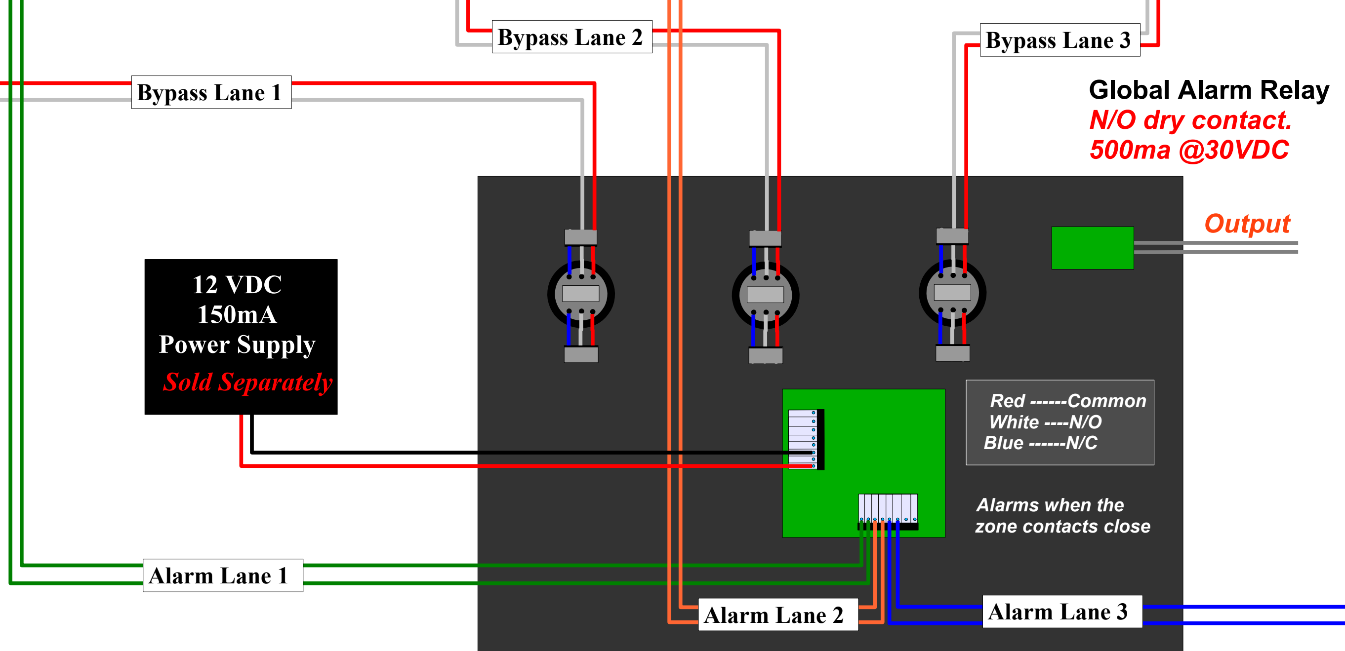
Desktop Controller (Back View)
